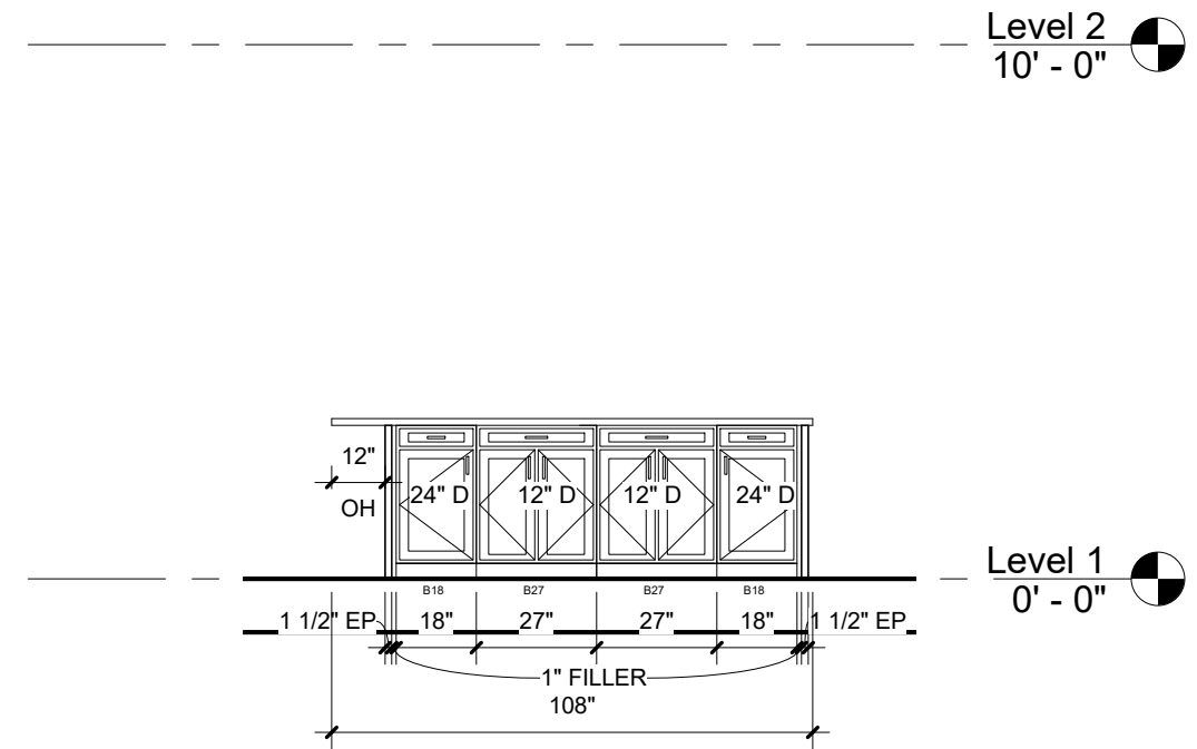
③ Elevation 1 - d 1/4" = 1'-0"
