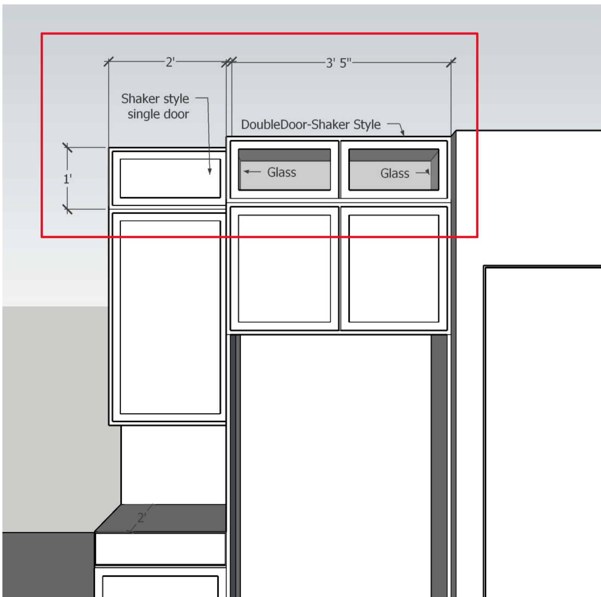
KITCHEN WALL 2 : UPPER CABINET
